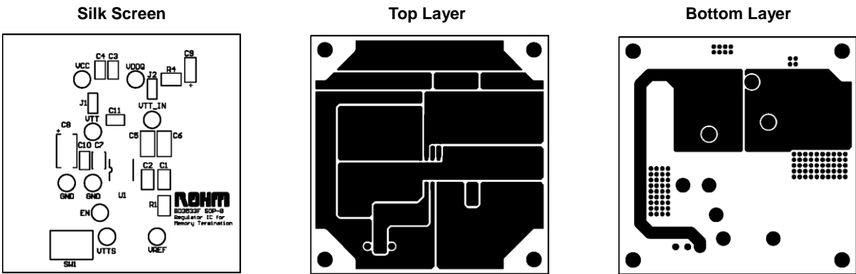
BD3533F (SOP8) Evaluation Board Layout
