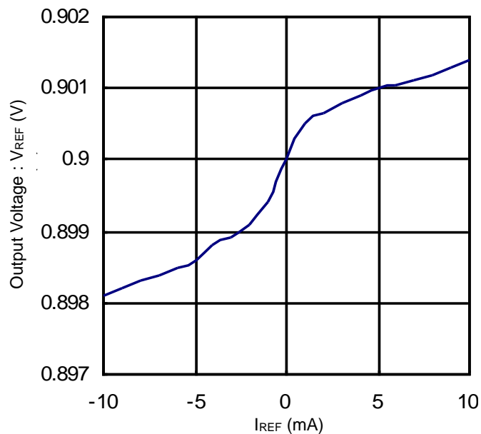
Figure 2. Output Voltage vs I_{REF} (DDR-2)
