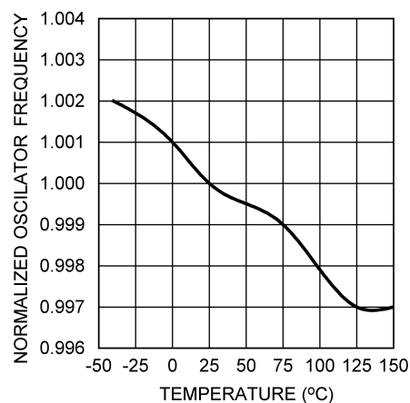
Figure 5-2. Oscillator Frequency vs Temperature (Q0) F_{Osc} = 200 \text{ kHz}
