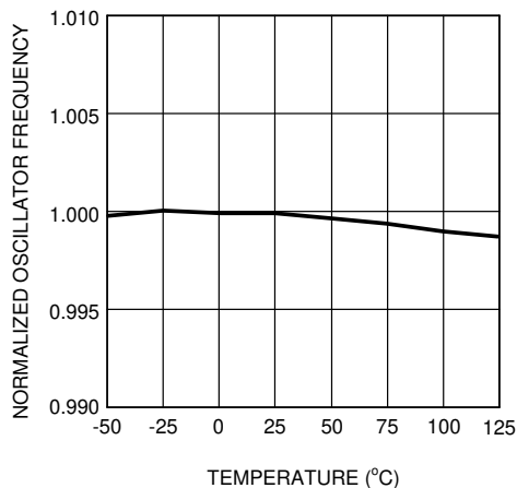
Figure 5-3. Oscillator Frequency vs Temperature (Q1) F_{Osc} = 200 \text{ kHz}
