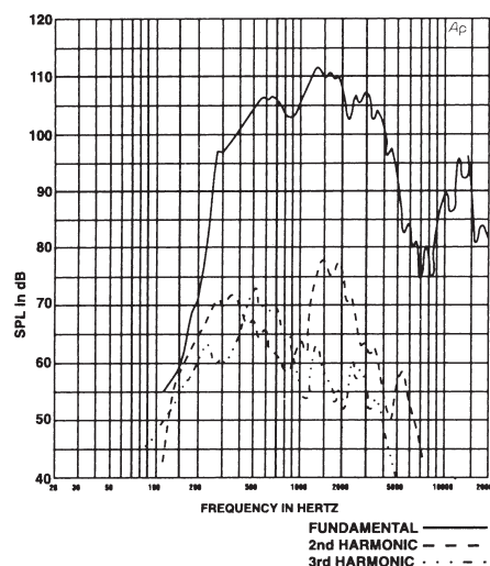
Figure 2. Distortion Response - FC100 Horn
