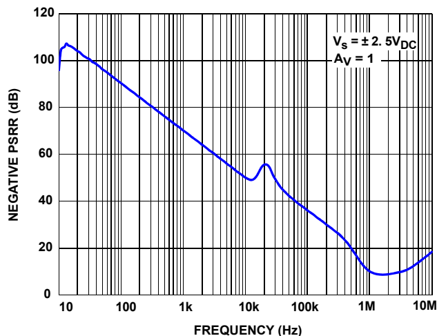
FIGURE 65. OP AMP POWER SUPPLY REJECTION RATIO
