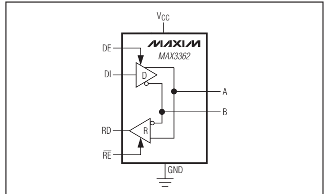
Functional Diagram
