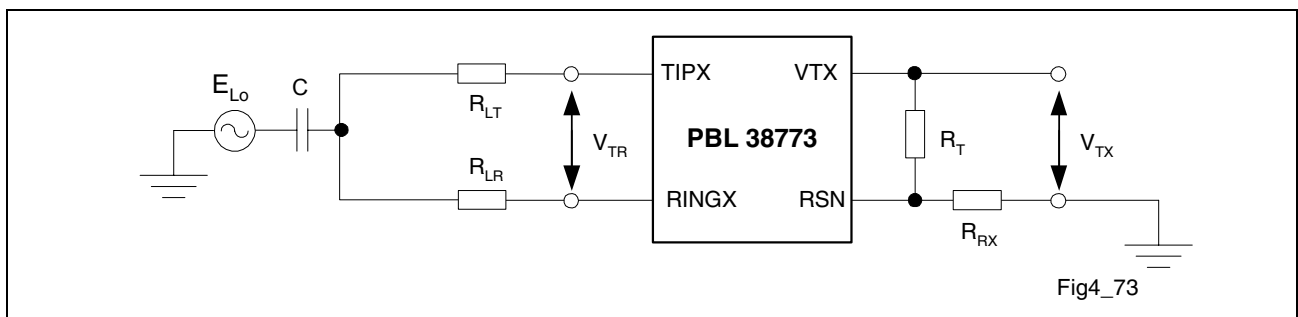
Figure 4 Longitudinal to Metallic, B_{LME} and Longitudinal to Four-Wire, B_{LFE} Balance
