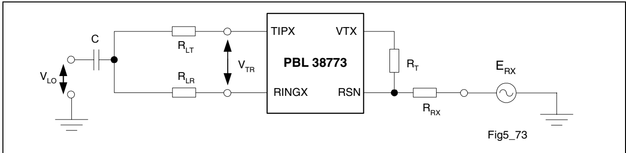
Figure 5 Metallic to Longitudinal, B_{MLE} and Four-Wire to Longitudinal Balance, B_{FLE}
