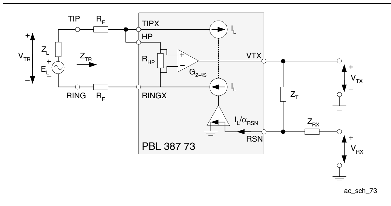
Figure 9 Simplified AC Model of PBL 38773/1
