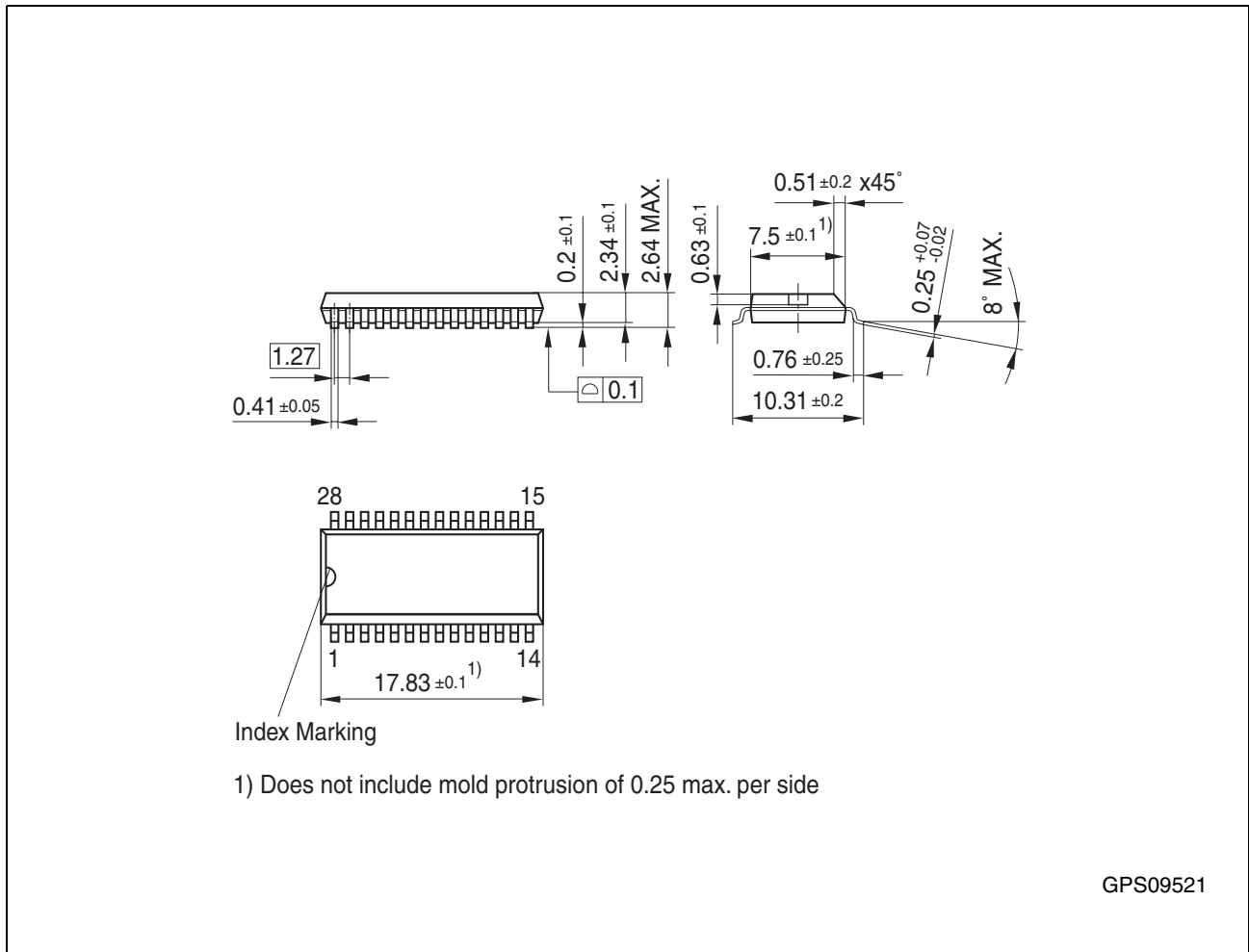
Figure 16 P-DSO-28-20 (Plastic Dual Small Outline Package)
