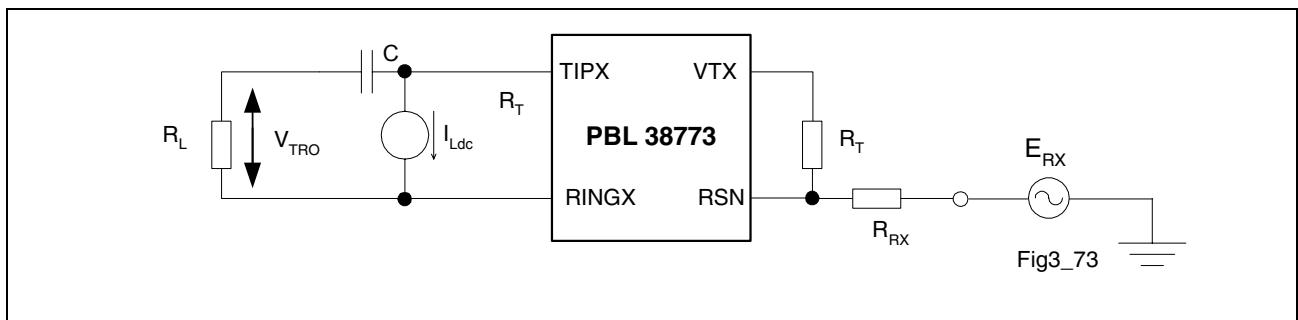
Figure 3 Overload Level, V_{TRO} , Two-Wire Port
