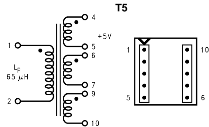
Figure 45. Schott 67140890 (Top View)
