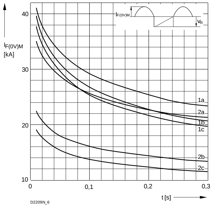
Bild / Fig. 4 Grenzstrom / Maximum overload forward current I_{F(0V)M} = f(t) 1 - I_{FAV(vor)} = 0\text{ A} ; t_{vj} = t_c = 25\text{ °C} 2 - I_{FAV(vor)} = 2200\text{ A} ; t_c = 100\text{ °C} ; t_{vj} = 160\text{ °C} a - V_R \leq 50\text{ V} b - V_R = 0,5 V_{RRM} c - V_R = 0,8 V_{RRM}
