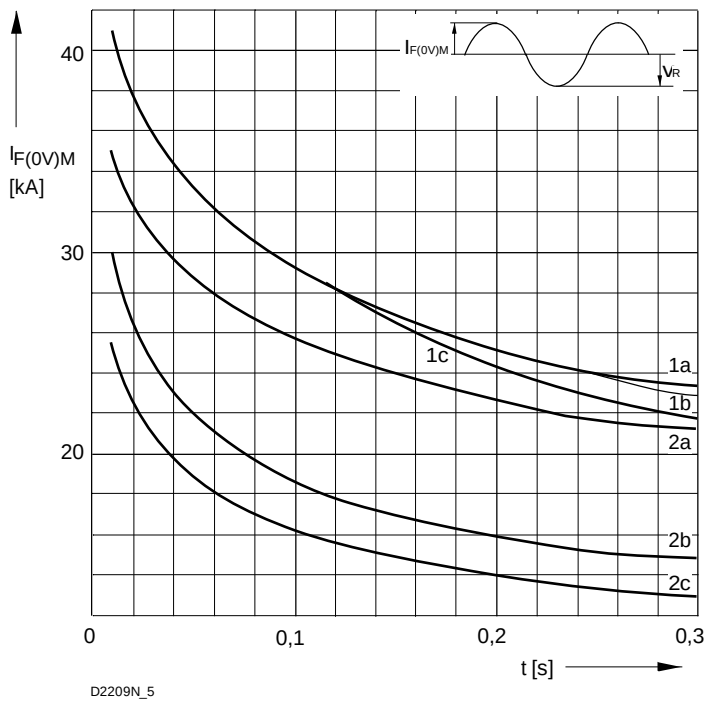
Bild / Fig. 3 Grenzstrom / Maximum overload forward current I_{F(0V)M} = f(t) 1 - I_{FAV(vor)} = 0\text{ A} ; t_{vj} = t_c = 25\text{ °C} 2 - I_{FAV(vor)} = 2200\text{ A} ; t_c = 100\text{ °C} ; t_{vj} = 160\text{ °C} a - V_R \leq 50\text{ V} b - V_R = 0,5 V_{RRM} c - V_R = 0,8 V_{RRM}
