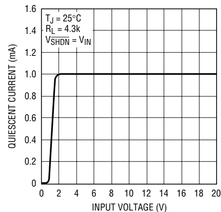
LT1764 Quiescent Current
