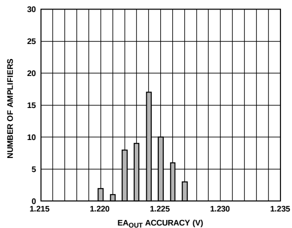
Figure 24. EA_{OUT} Accuracy Voltage Distribution at -40°C
