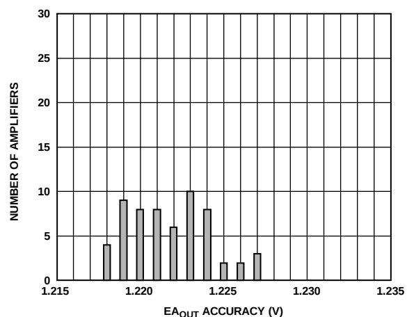
Figure 23. EA_{OUT} Accuracy Voltage Distribution at 125°C
