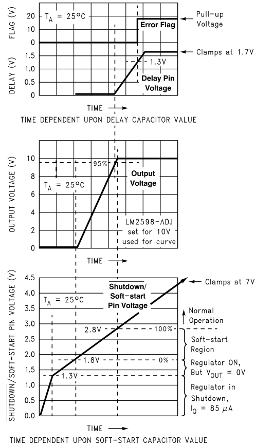
Figure 30. Soft-start, Delay, Error, Output
