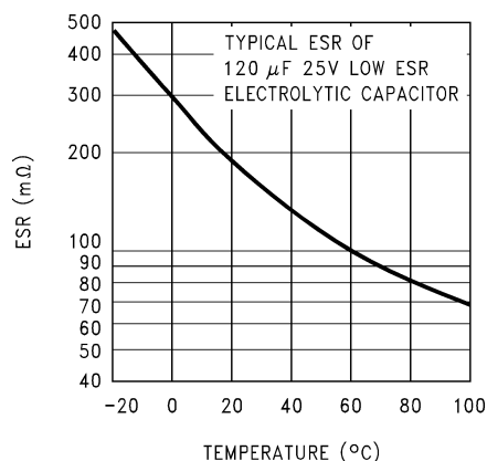
Figure 35. Capacitor ESR Change vs Temperature
