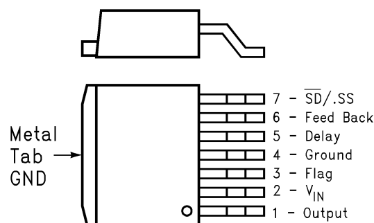
Figure 2. 7-Lead Surface Mount DPAK (S) Package See Package Number KTW0007B
