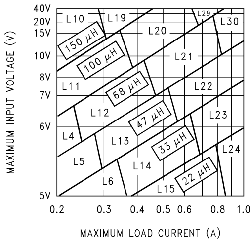
Figure 25. LM2598-3.3
