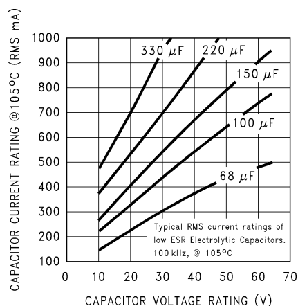
Figure 33. RMS Current Ratings for Low ESR Electrolytic Capacitors (Typical)
