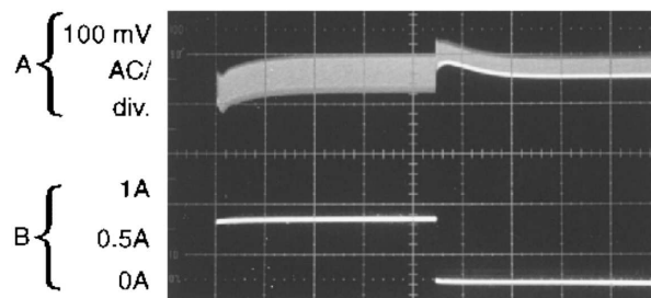
Figure 23. Horizontal Time Base: 200 \mu\text{s}/\text{div} .
