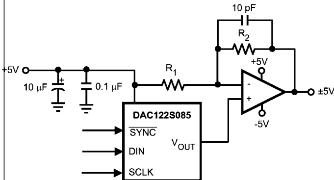
FIGURE 9. Bipolar Operation
