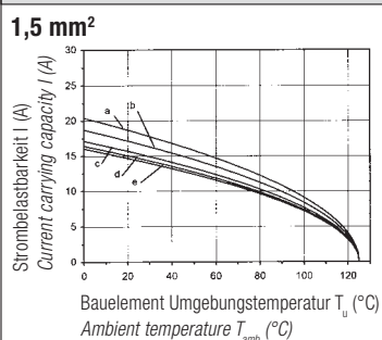
Derating Kurven / Derating curves
