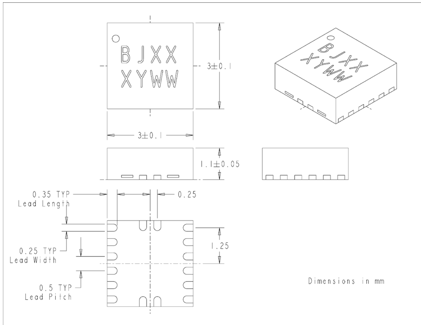
Figure 12. EP53A8LQA Package Dimensions (Bottom View)
