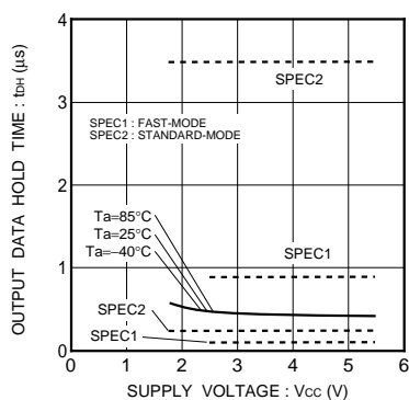
Fig.39 Output data hold time t_{di0}
