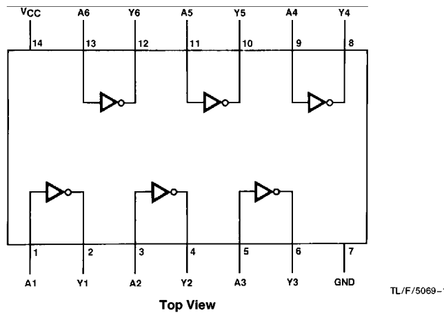
Dual-In-Line Package
