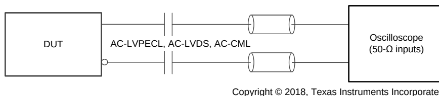
Figure 17. AC-LVPECL, AC-LVDS, AC-CML Output AC Test Configuration
