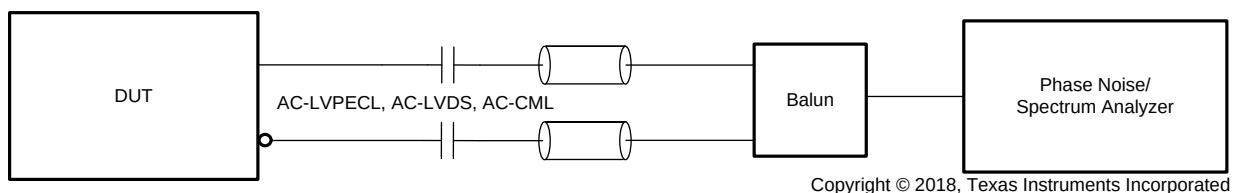
Figure 18. AC-LVPECL, AC-LVDS, AC-CML Output Phase Noise Test Configuration
