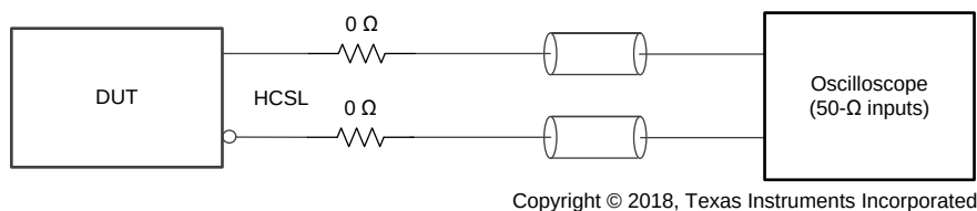
Figure 19. HCSL Output Test Configuration
