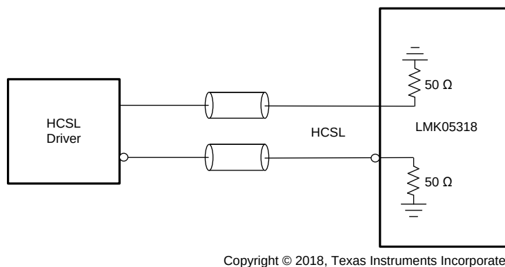
Figure 34. HCSL (Load Terminated) to Reference (PRIREF/SECREF) or XO Inputs
