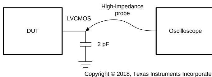
Figure 15. LVC MOS Output Test Configuration
