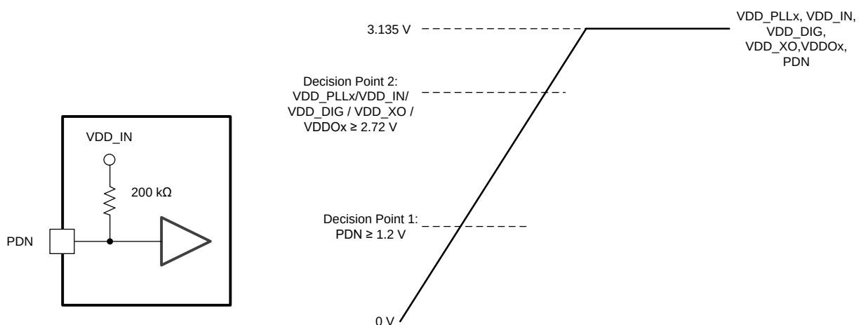
Figure 62. Recommendation for Power Up From a Single-Supply Rail
