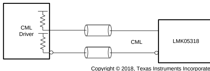
Figure 33. DC-Coupled CML (Source Terminated) to Reference (PRIREF/SECREF) or XO Inputs
