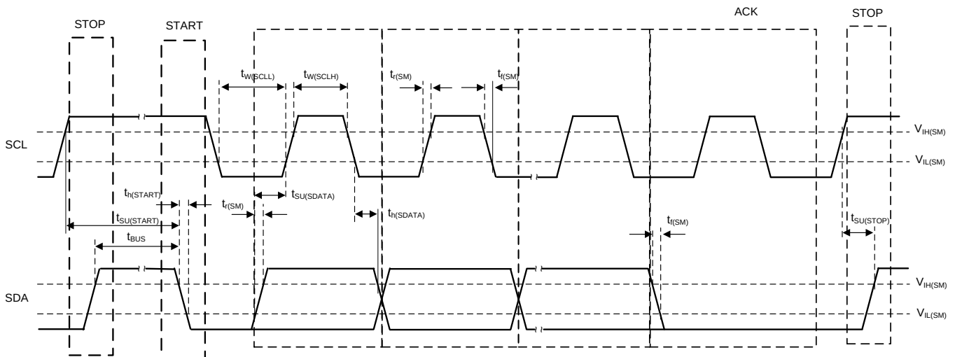
Figure 3. I²C Timing Diagram
