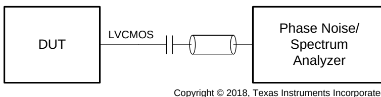
Figure 16. LVC MOS Output Phase Noise Test Configuration
