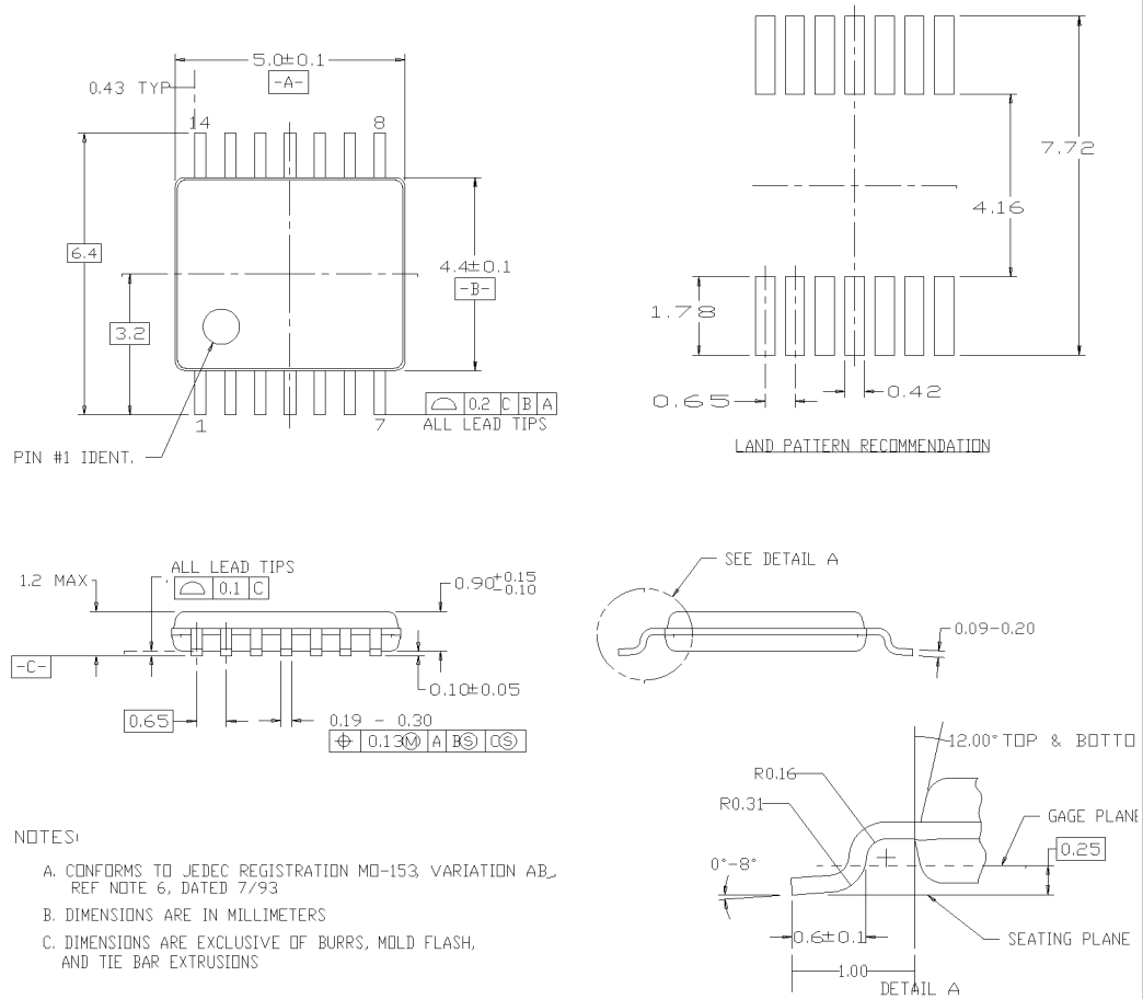
14-Thin Shrink Small Outline Package (TSSOP), JEDEC MO-153, 4.4mm Wide Package Number MTC14
