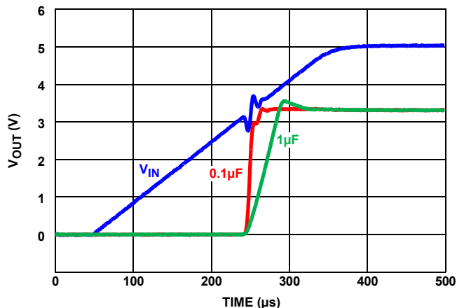
FIGURE 114. TURN-ON TIME
