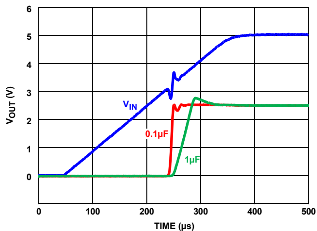
FIGURE 80. TURN-ON TIME
