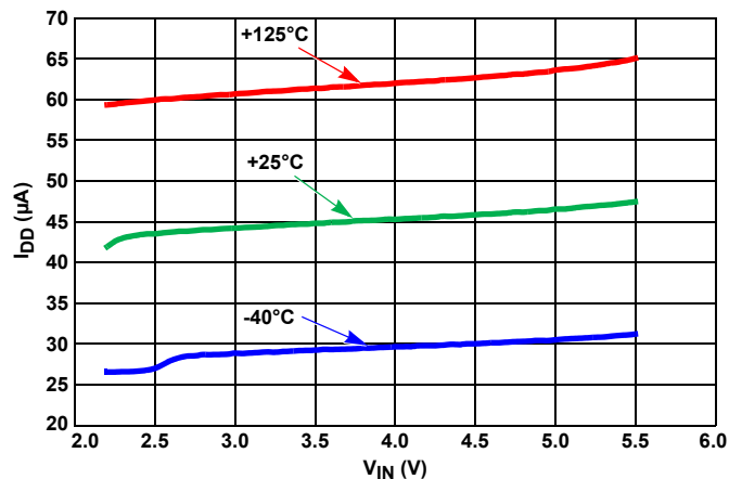
FIGURE 55. I_{DD} vs V_{IN} , OVER-TEMPERATURE
