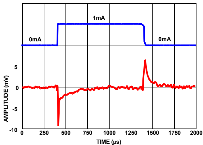
FIGURE 130. LOAD TRANSIENT RESPONSE AT 1mA LOAD AT 1\mu F
