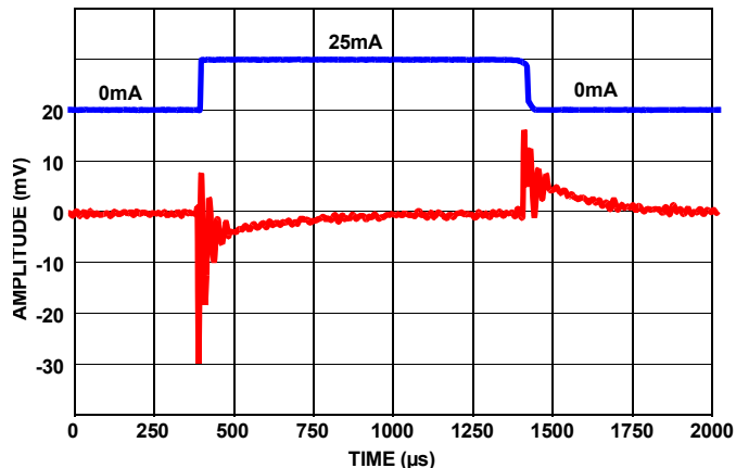
FIGURE 129. LOAD TRANSIENT RESPONSE AT 25mA LOAD AT 1\mu F
