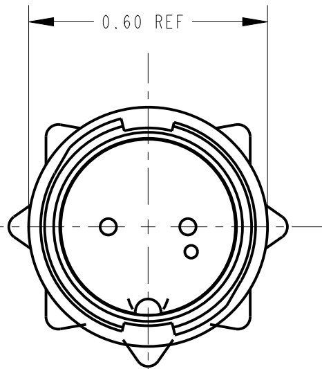
CUSTOMER DRAWING
