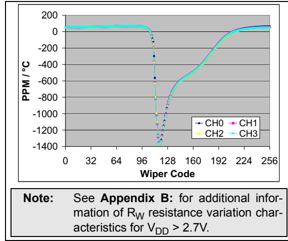
FIGURE 2-41: 10 kΩ – R_{WB} PPM/°C vs. Wiper Setting. ( R_{BW(\text{code}=n, 125^\circ\text{C})} - R_{BW(\text{code}=n, -40^\circ\text{C})} / R_{BW(\text{code}=256, 25^\circ\text{C})} / 165^\circ\text{C} * 1,000,000 ) ( V_{DD} = 1.8\text{V} , I_W = 150\text{ }\mu\text{A} ).
