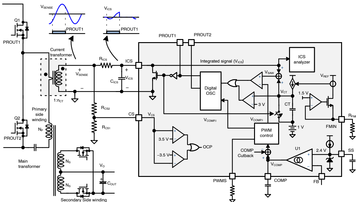
Figure 83. Basic Application Circuit for Current Sensing and Soft-Start
