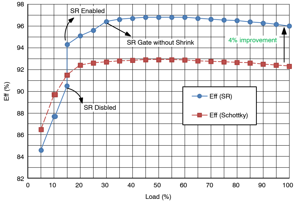
Figure 84. Evaluation Board (EVB) Measured Efficiency
