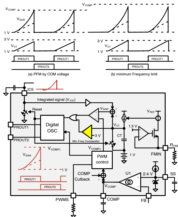
Figure 74. Minimum Switching Frequency Setting
