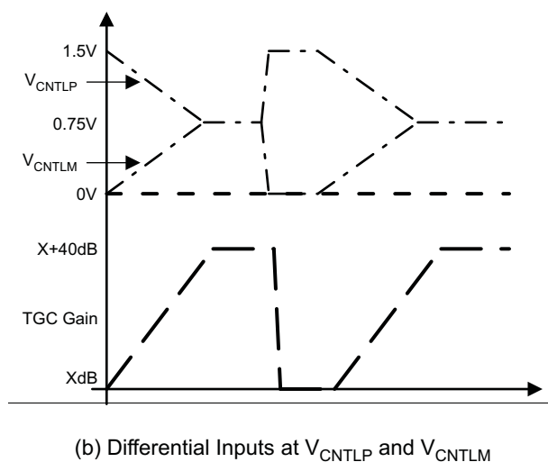
Figure 85. V_{CNTLP} and V_{CNTLM} Configurations
