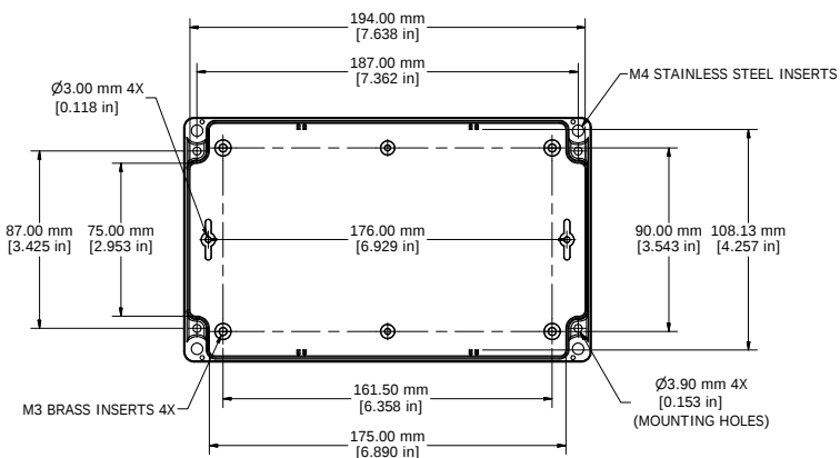
BOX - INSIDE
