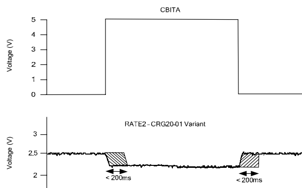
Figure 10 - CBITA Timing
