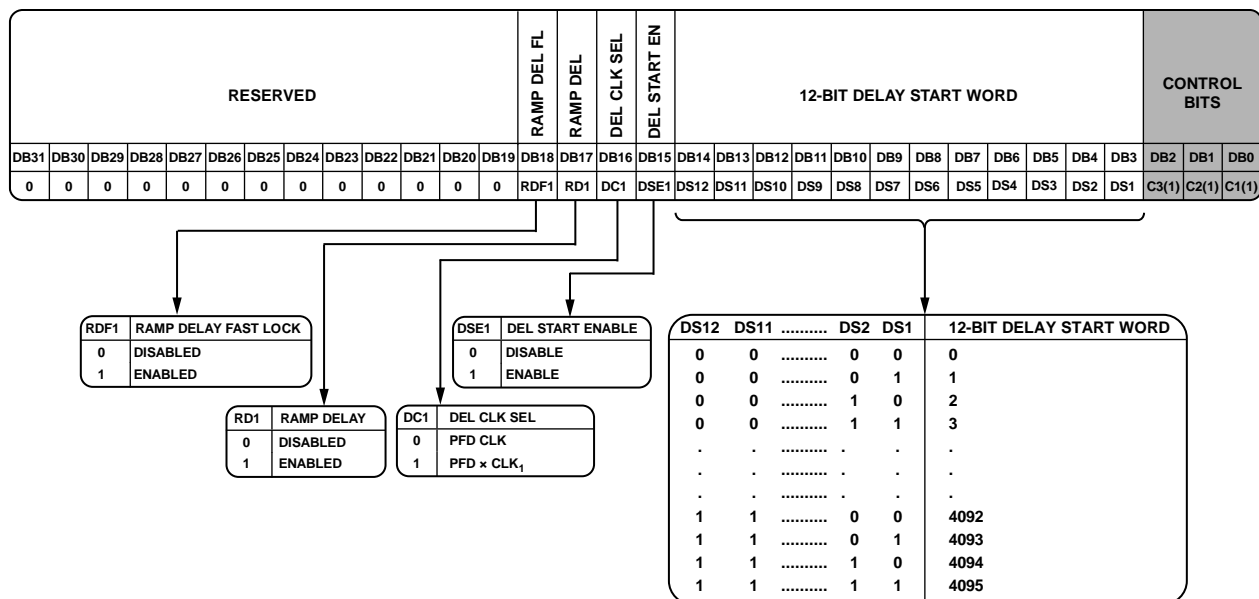
Figure 30. Delay Register (R7) Map
