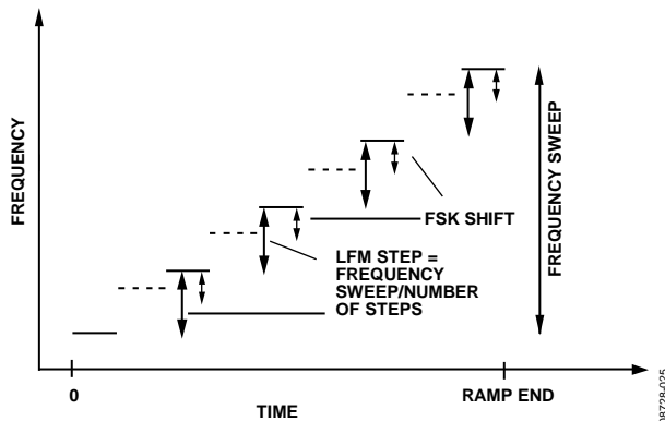
Figure 37. Combined FSK and LFM Waveform (N Corresponds to the Number of LFM Steps)
