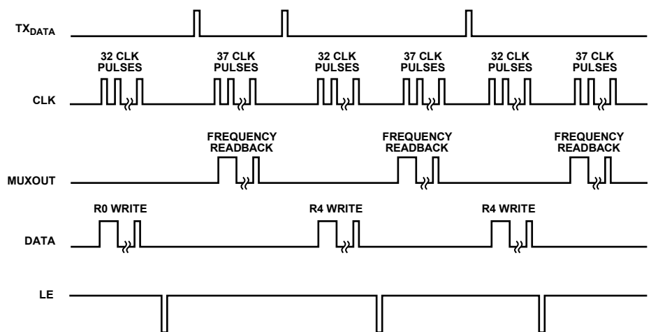
Figure 44. Continuous Frequency Readback
