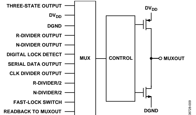
Figure 20. MUXOUT Schematic
