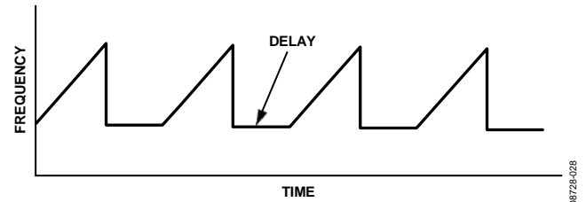
Figure 39. Delay Between Ramps for Sawtooth Mode
