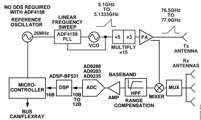
Figure 47. FMCW Radar with ADF4158
