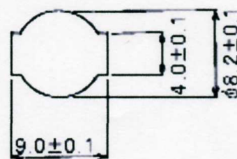
Shape of Mounting Hole
