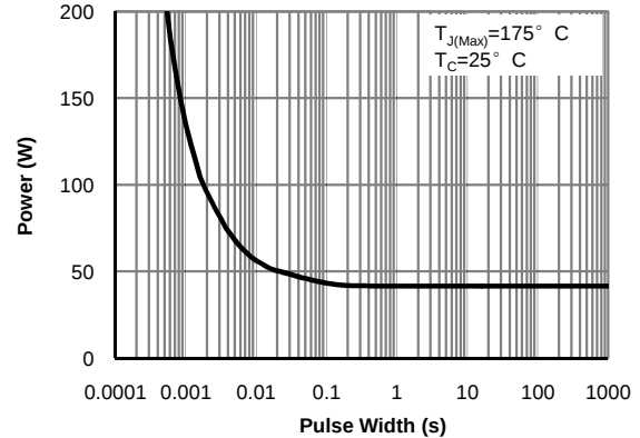
Figure 10: Single Pulse Power Rating Junction-to-Case for AOT2618L and AOB2618L (Note F)
