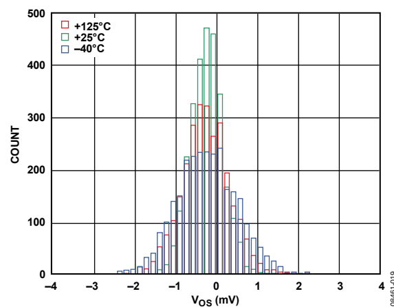
Figure 20. Offset Distribution
