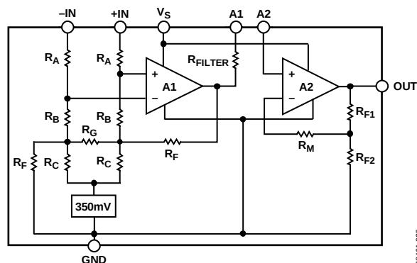
Figure 23. Simplified Schematic
