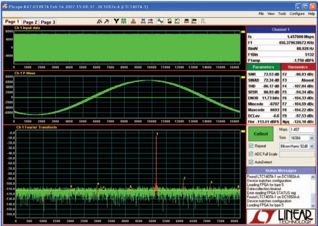
Figure 2. DC1082A Screenshot
