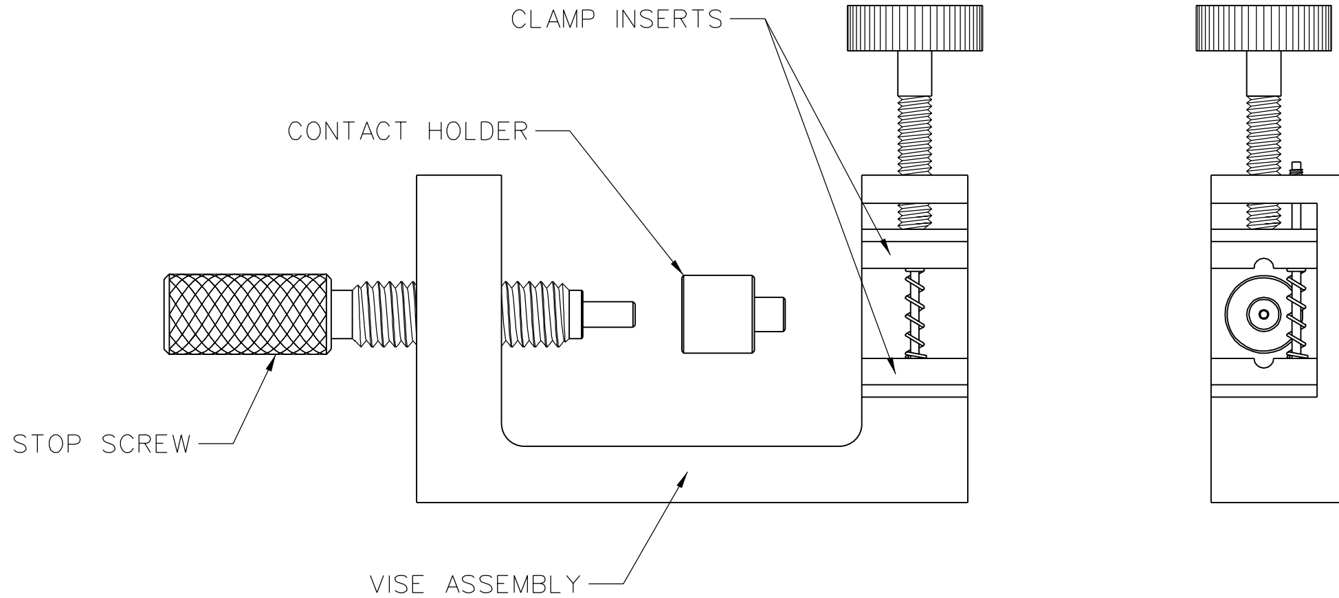
CABLE VISE APPLICATION 1.5:1 (FOR REFERENCE ONLY)
