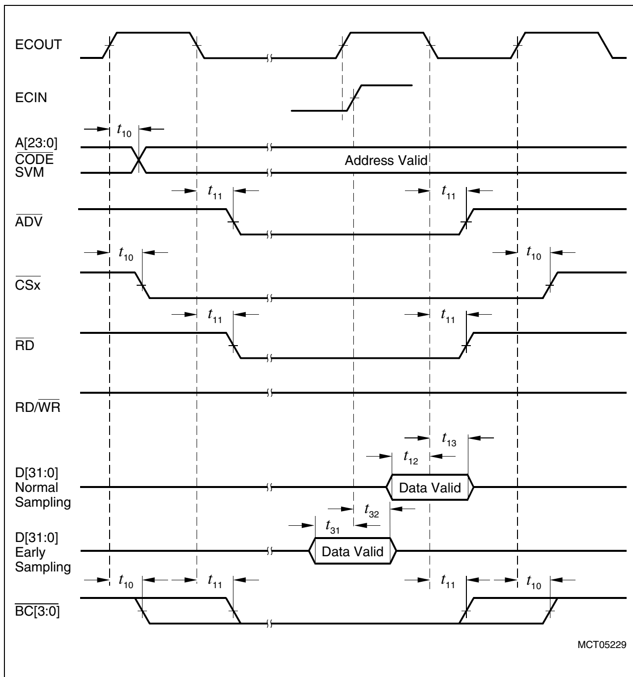
Figure 30 EBU Demultiplexed Read Timing
