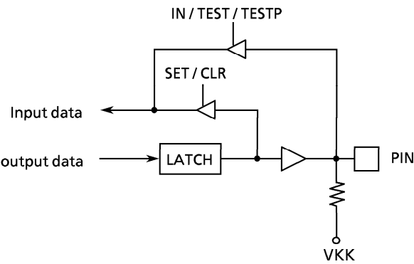
Figure 3-4. R4, R5, R6 port
