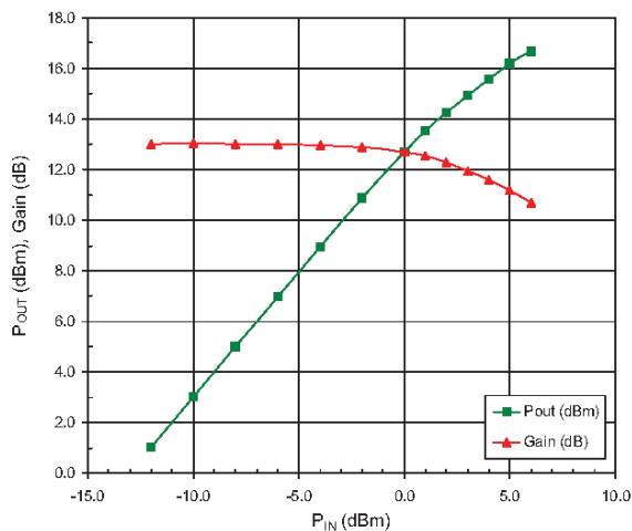
P_{OUT}/\text{Gain} versus P_{IN} at 14 GHz
