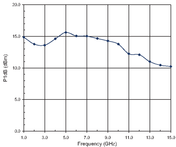
P1dB versus Frequency at 25°C
