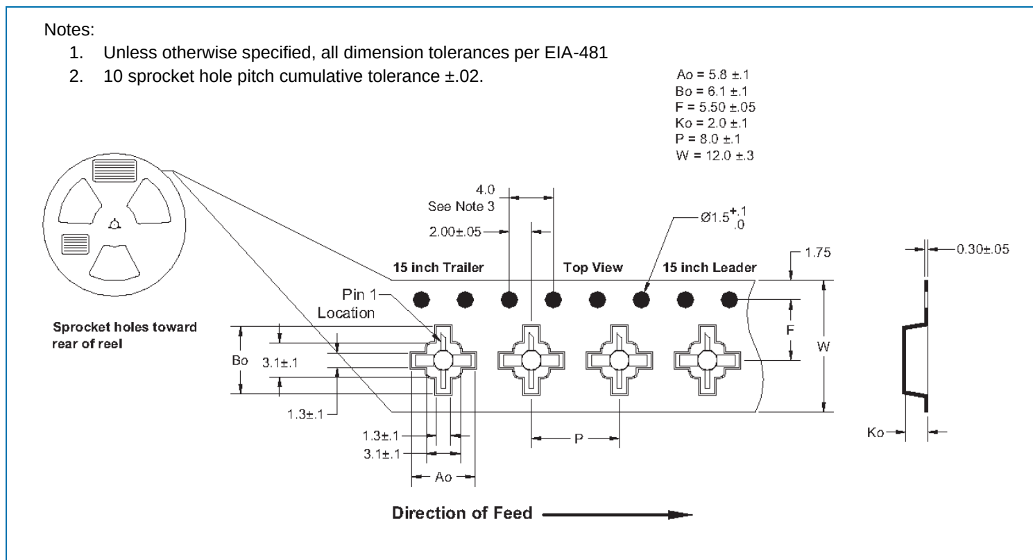
Figure 1. Carrier Tape Drawing with Part Orientation
