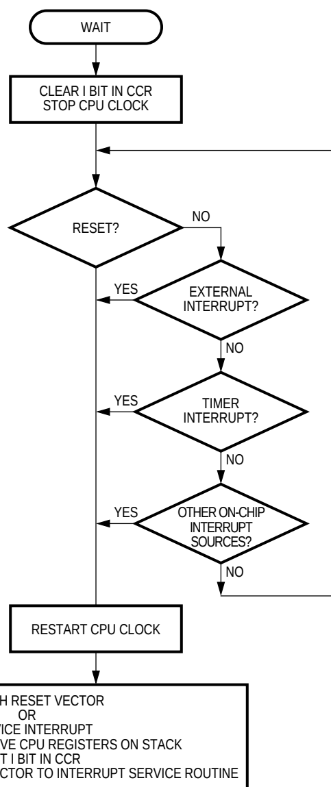
Figure 26. WAIT Instruction Flowchart
