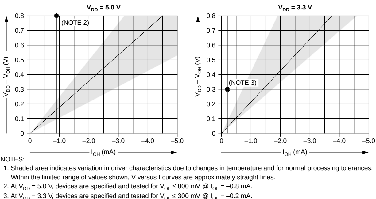
Figure 70. Typical High-Side Driver Characteristics
