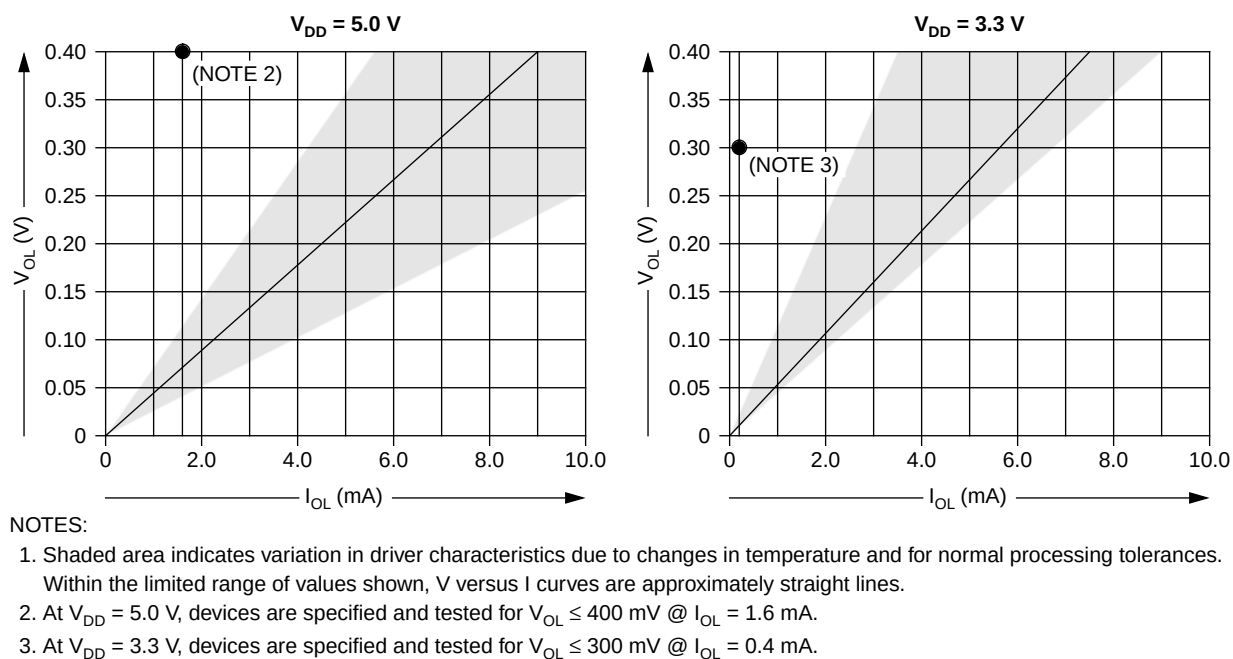
Figure 71. Typical Low-Side Driver Characteristics
