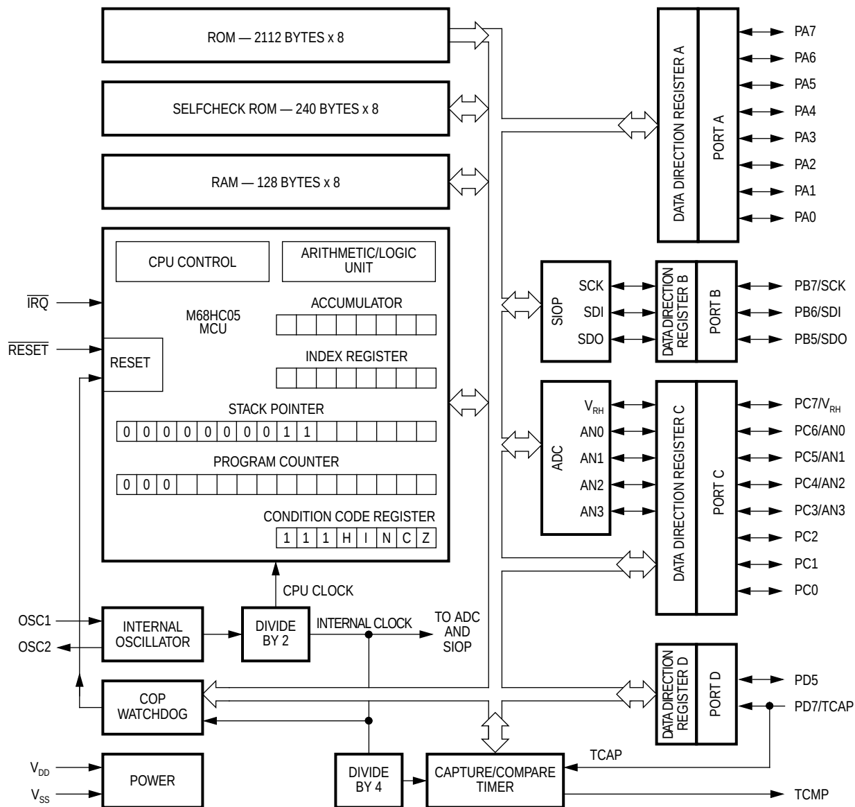
Figure 1. MC68HC05P9A Block Diagram
