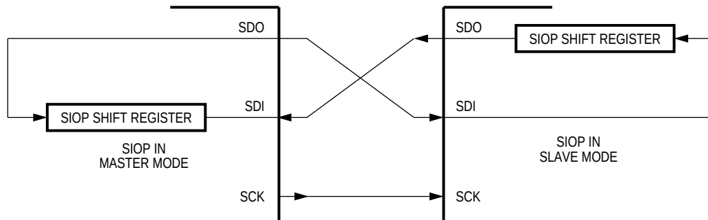
Figure 62. Master/Slave SIOP Shift Register Operation
