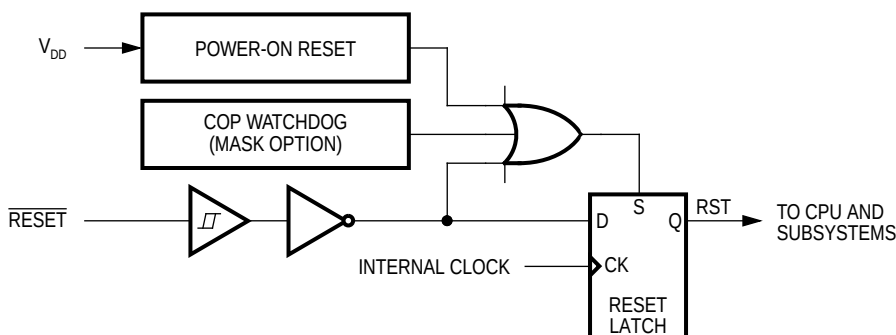
Figure 17. Reset Sources
