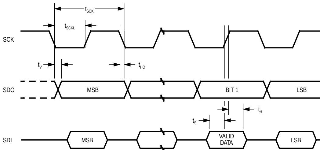
Figure 63. SIOF Timing
