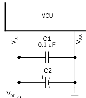
Figure 3. Bypassing Recommendation
