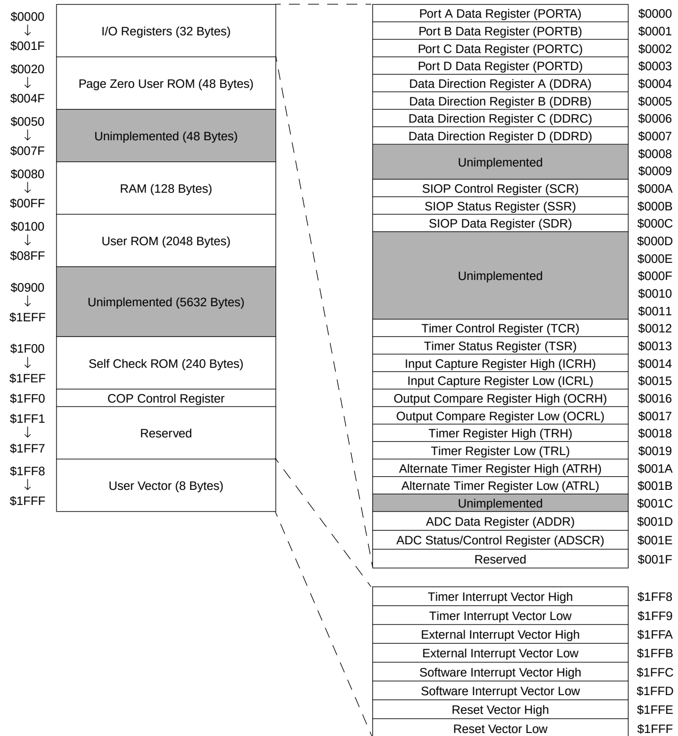
Figure 8. Memory Map
