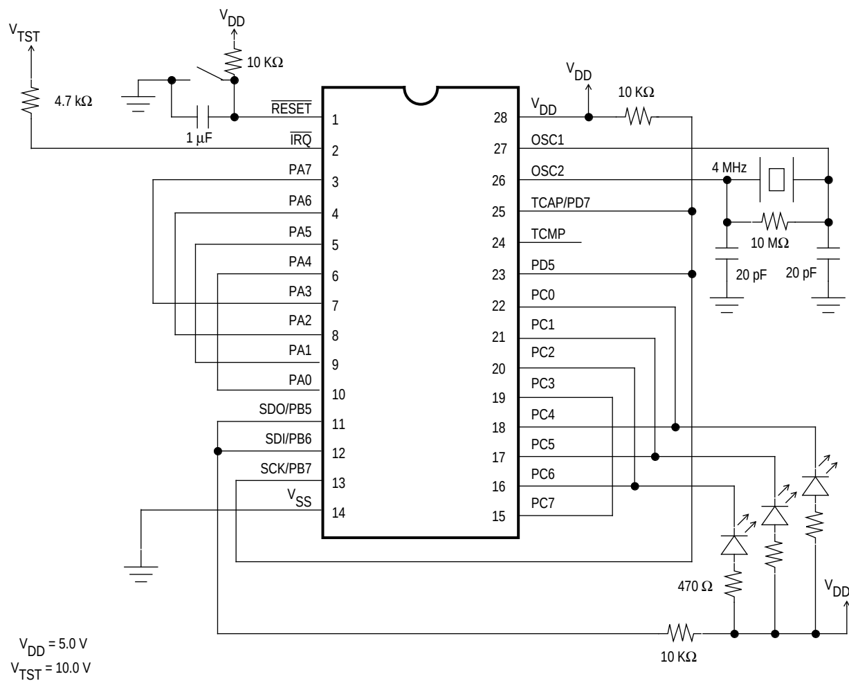
Figure 10. Self-Check Circuit
