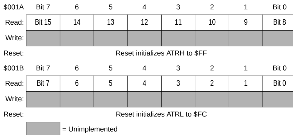
Figure 55. Alternate Timer Registers (ATRH and ATRL)
