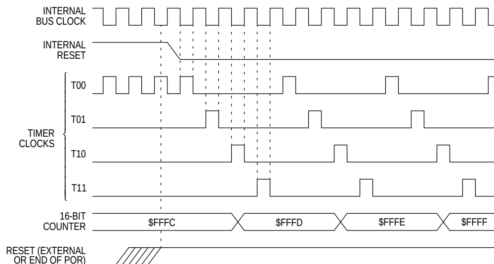
Figure 47. Timer Reset Timing
