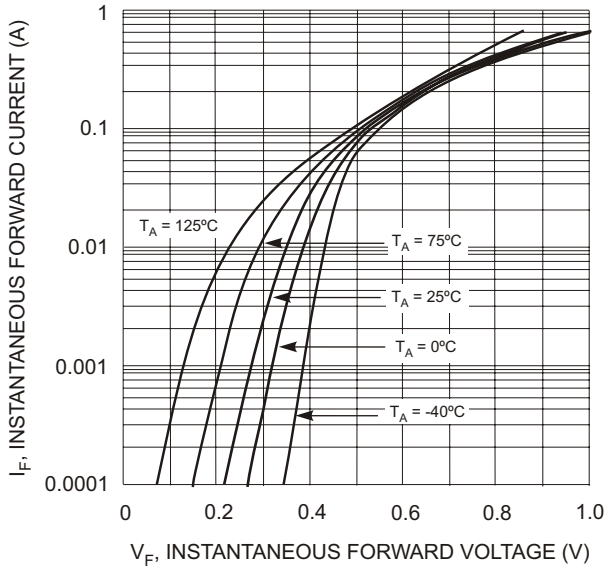
Fig. 1 Forward Characteristics
