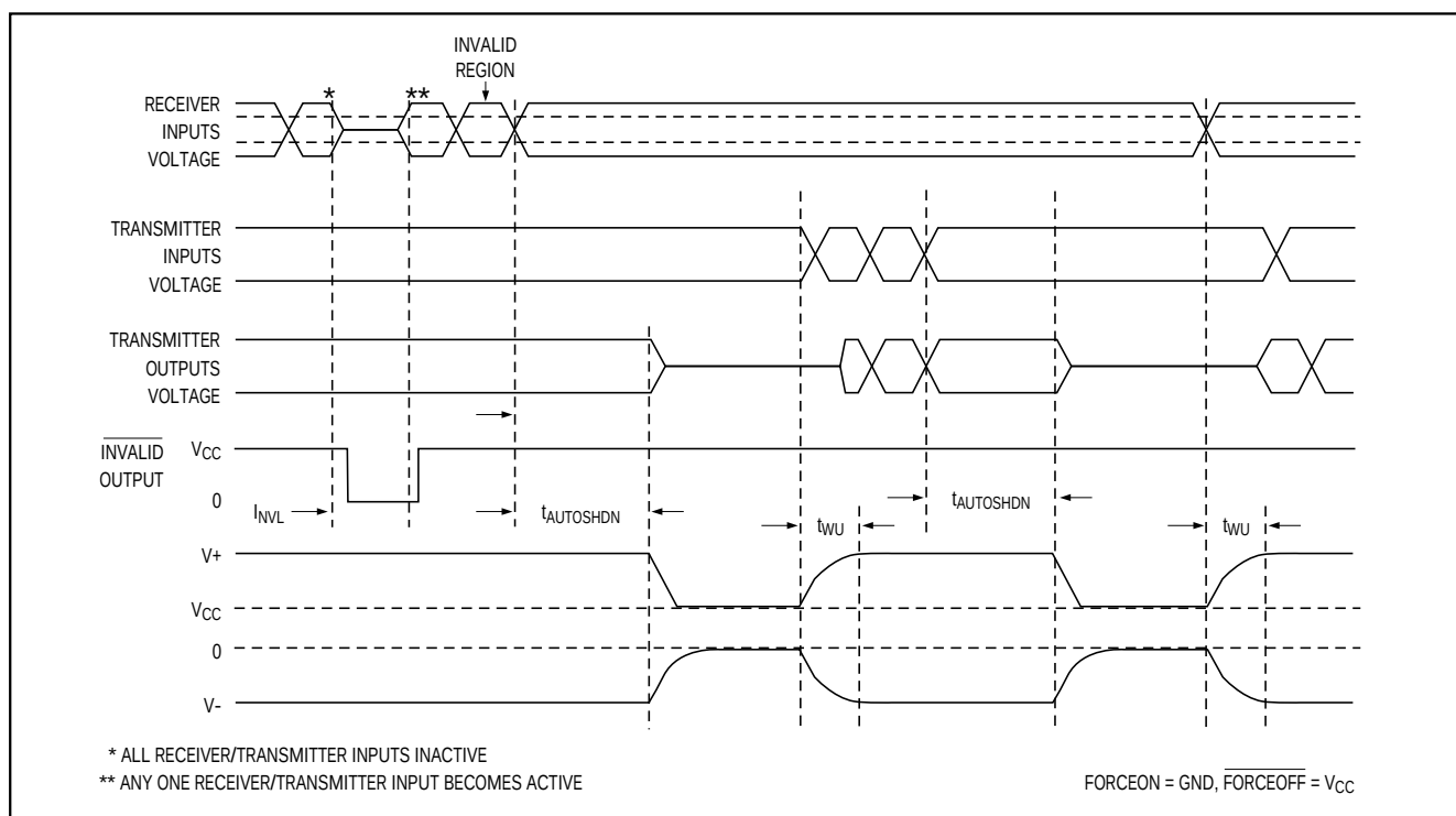
Figure 3a. AutoShutdown Plus and \overline{\text{INVALID}} Timing Diagram
