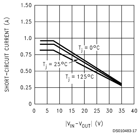
Short-Circuit Current
