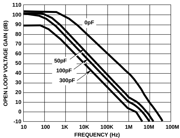
FIGURE 8. OPEN LOOP FREQUENCY RESPONSE FOR VARIOUS COMPENSATION CAPACITANCES
