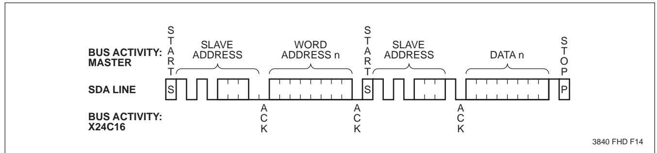
Figure 8. Random Read
