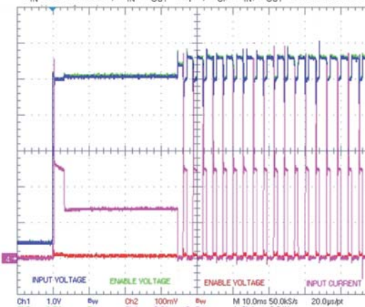
Figure 20. Soft-start behavior (5 V)
