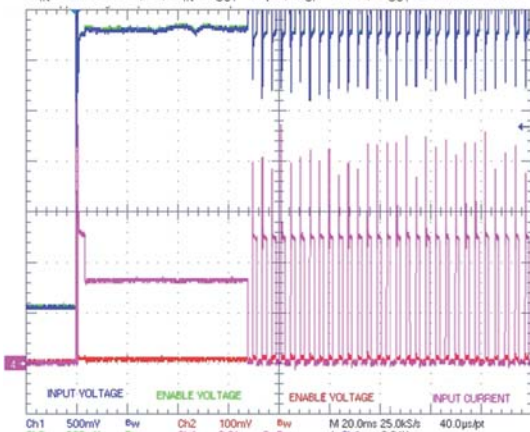
Figure 19. Soft-start behavior (3.3 V)
