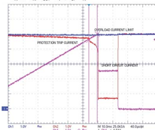
Figure 18. Startup into short-circuit (5 V)
