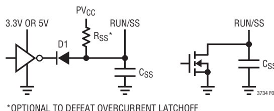
Figure 3. RUN/SS Pin Interfacing
