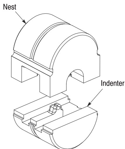
Flag Terminal Die Set (Typical)
