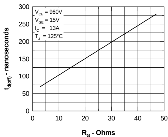
Fig. 8 Typ. Turn Off Delay Time
