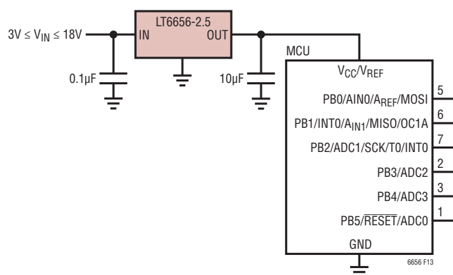
Figure 13. Microcontroller Reference and Regulator
