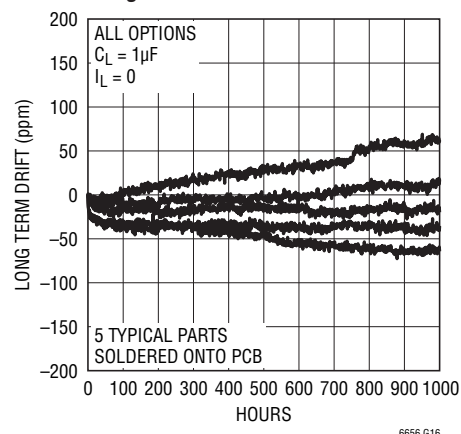
Long-Term Drift
