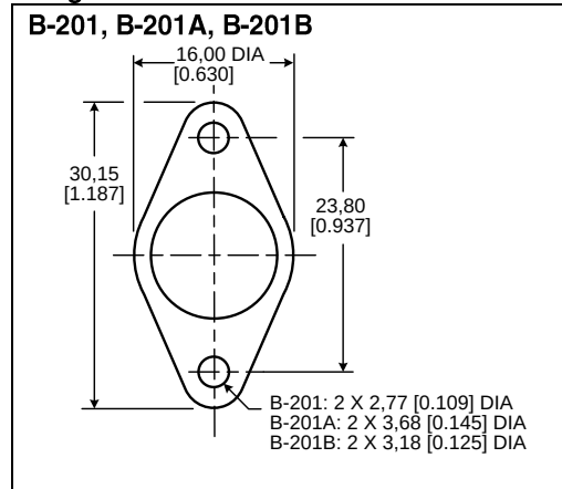
Figure 19. 3001/3004 Brackets
