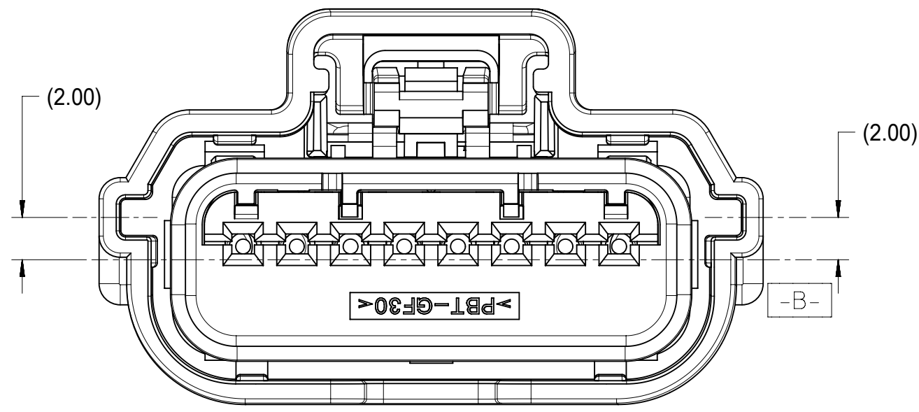
POLARIZATION A
