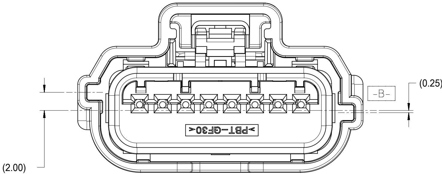
POLARIZATION C
