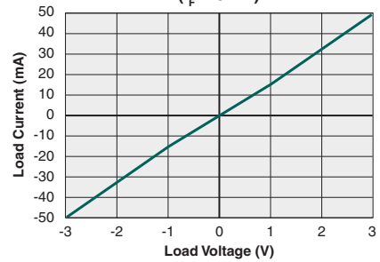
Typical Load Current vs. Load Voltage ( I_F=10mA )
