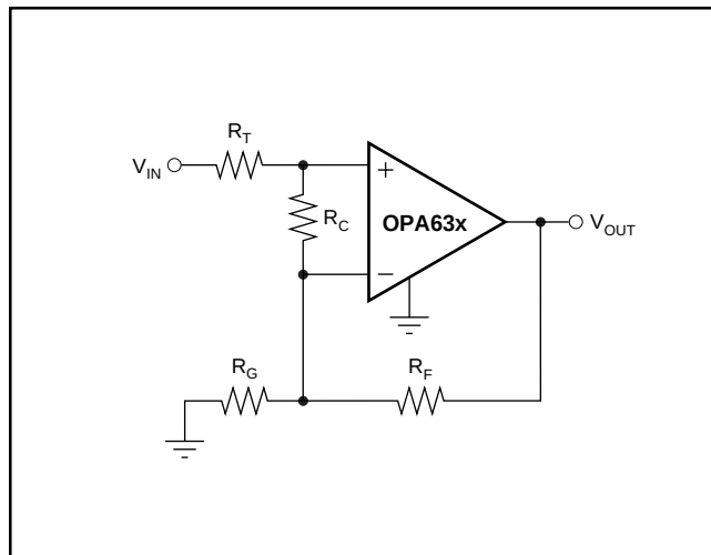
FIGURE 4. Compensated Non-Inverting Amplifier.
