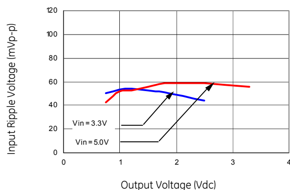
Figure 28. Input ripple voltage for various output with 2x150 μF polymer and 2x47 μF ceramic capacitors at the input (full load).
