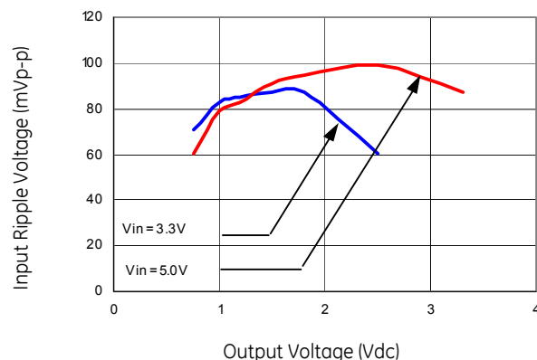
Figure 27. Input ripple voltage for various output with 1x150 μF polymer and 1x47 μF ceramic capacitors at the input (full load).
