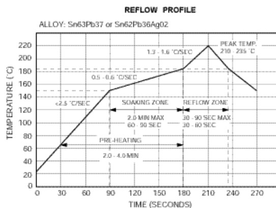
Figure 37. Reflow Profile.
