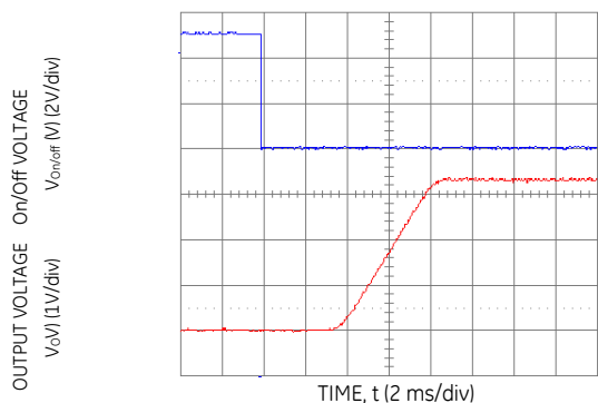
Figure 16. Typical Start-Up Using Remote On/Off with Low-ESR external capacitors (7x150uF Polymer) ( V_{in} = 5.0 Vdc, V_o = 3.3 Vdc, I_o = 5.0 A, C_o = 1050 \mu F).
